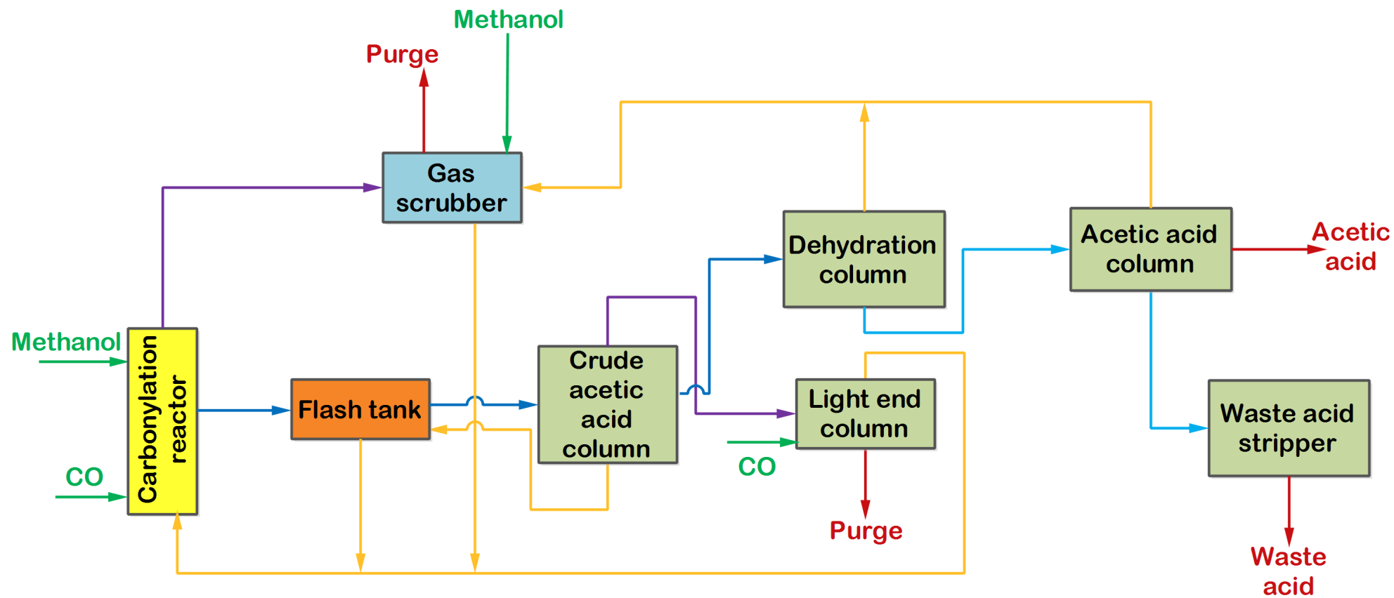
Figure: Manufacture of acetic acid by methanol carbonylation
